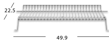
Porcelain Coated Warming Rack 1,097 Sq. Cm.
